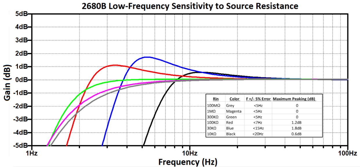
Figure 1: Source Resistance
